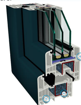
GEALAN S 9000
